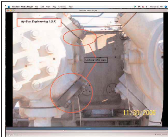
At one compressor station, the infrared camera showed gas billowing out of the valve caps and outer head of a reciprocating compressor.
