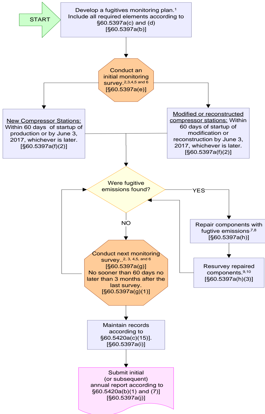
Figure 2. Fugitive Emissions Monitoring and Repair Requirements for the Collection of Fugitive Emissions Components at Compressor Stations
